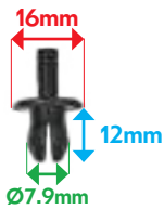
VB4000705 AGRAFE TOLE AUVENT
