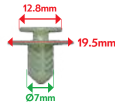
VB12014 MOULURE PB Scenic III
